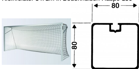
Kleinfeldtor 3 x 2m in Bodenhülsen Haspo 150
